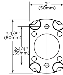
Snap Flange
